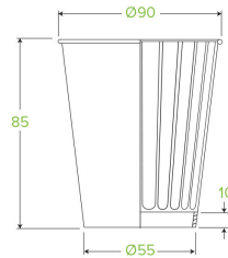
Double Wall 8 oz UNI
