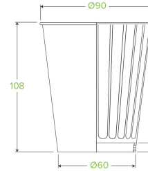
Double Wall 12 oz
