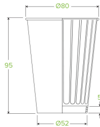
Double Wall 8 oz
